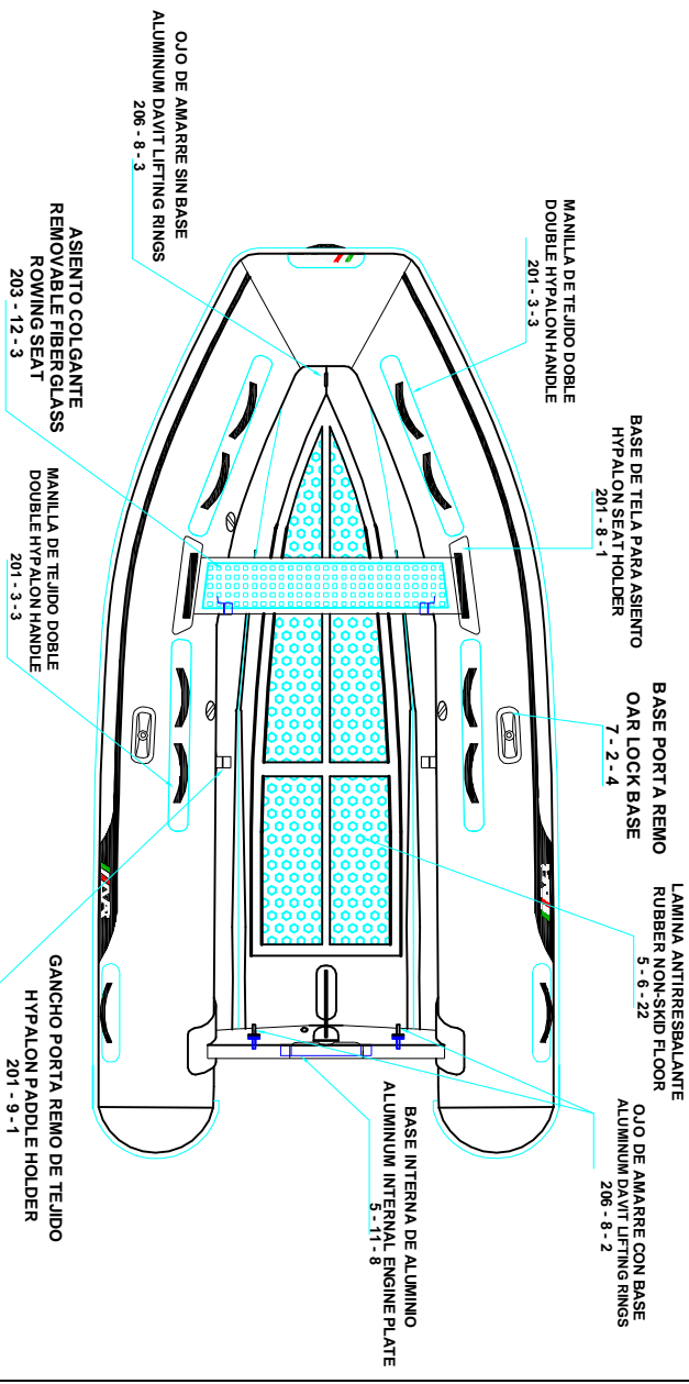
PLANT VIEW VISTA SUPERIOR
