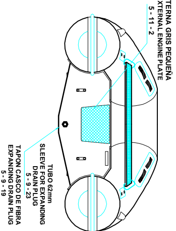
AFT VIEW VISTA TRASERA
