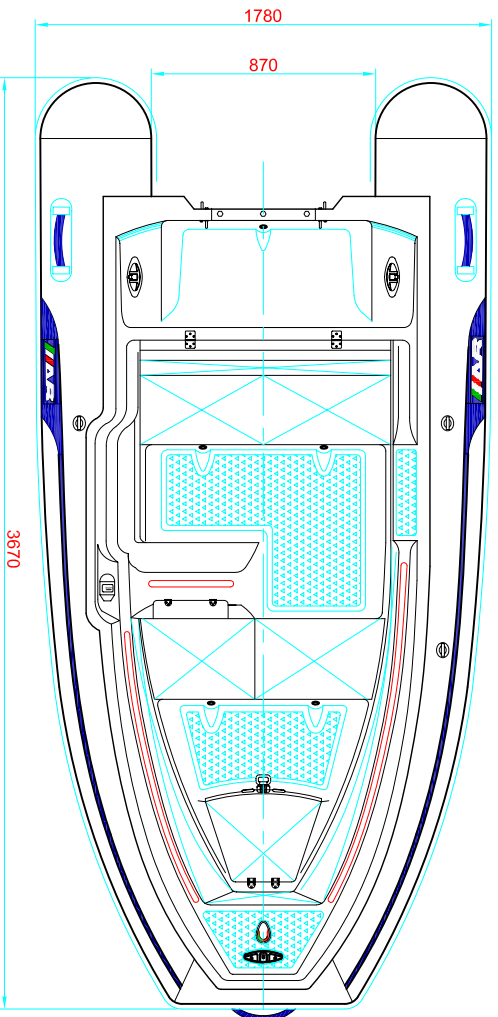
PLANT VIEW
