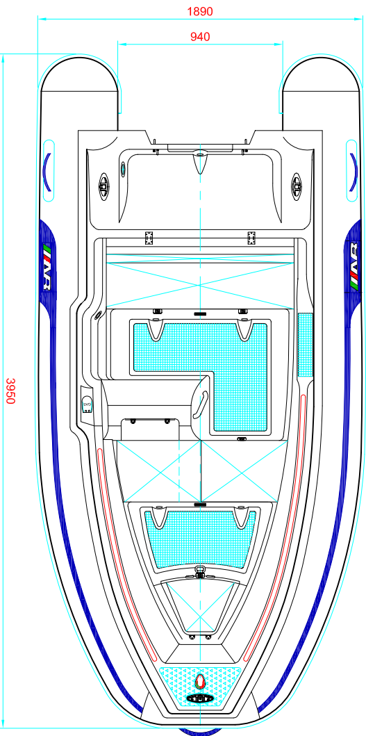
PLANT VIEW
