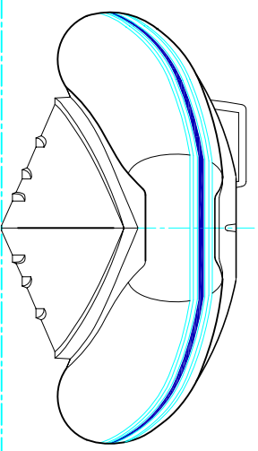
AFT VIEW
