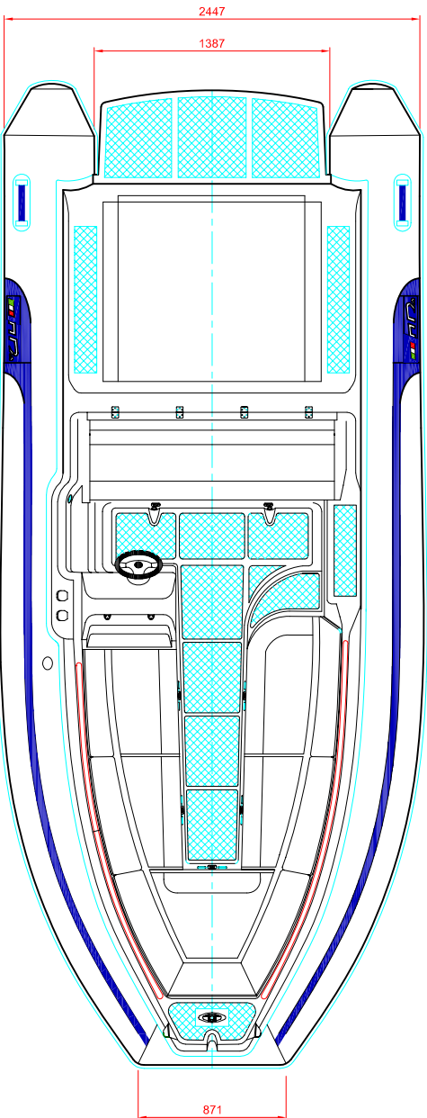
PLANT VIEW
