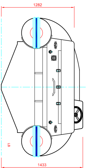
FORE VIEW
