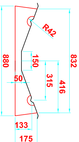
TRANSVERSAL SECTION "A" SECCION TRANSVERSAL "A"
