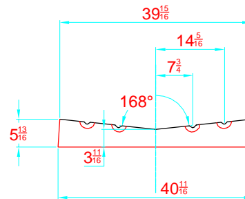
TRANSVERSAL SECTION "A" SECCION TRANSVERSAL "A"
