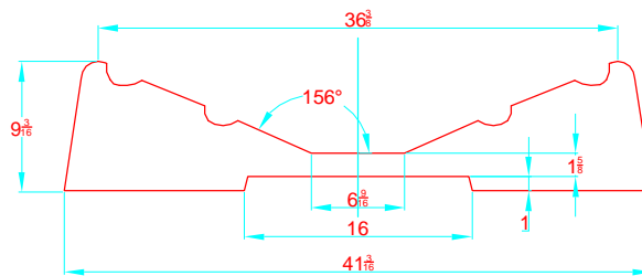
TRANSVERSAL SECTION "A" SECCION TRANSVERSAL "A"
