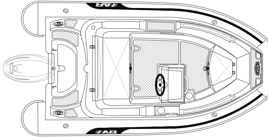
PLANT VIEW
