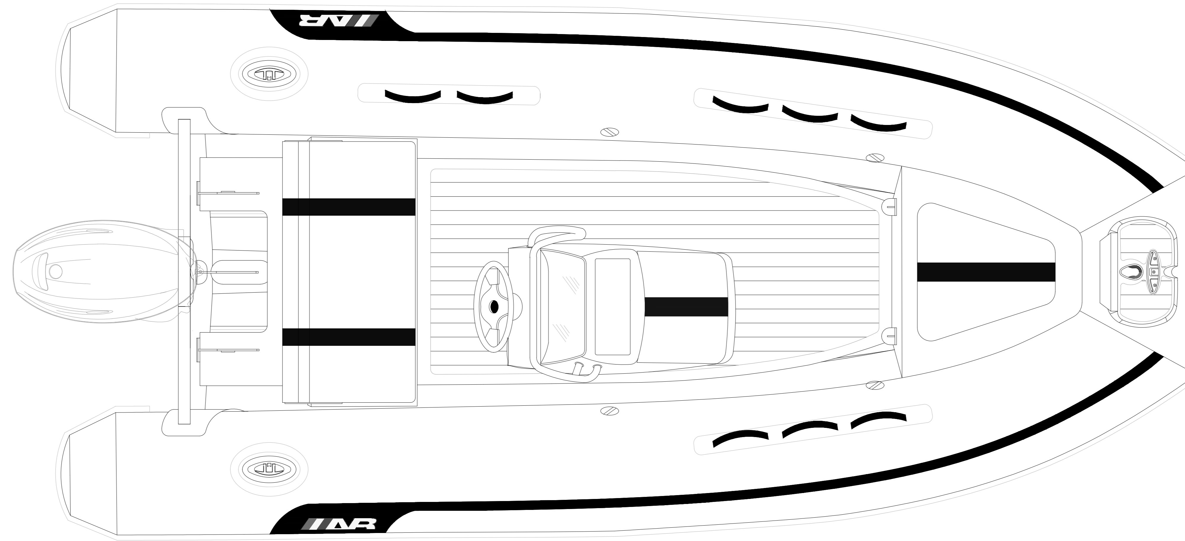
PLANT VIEW
