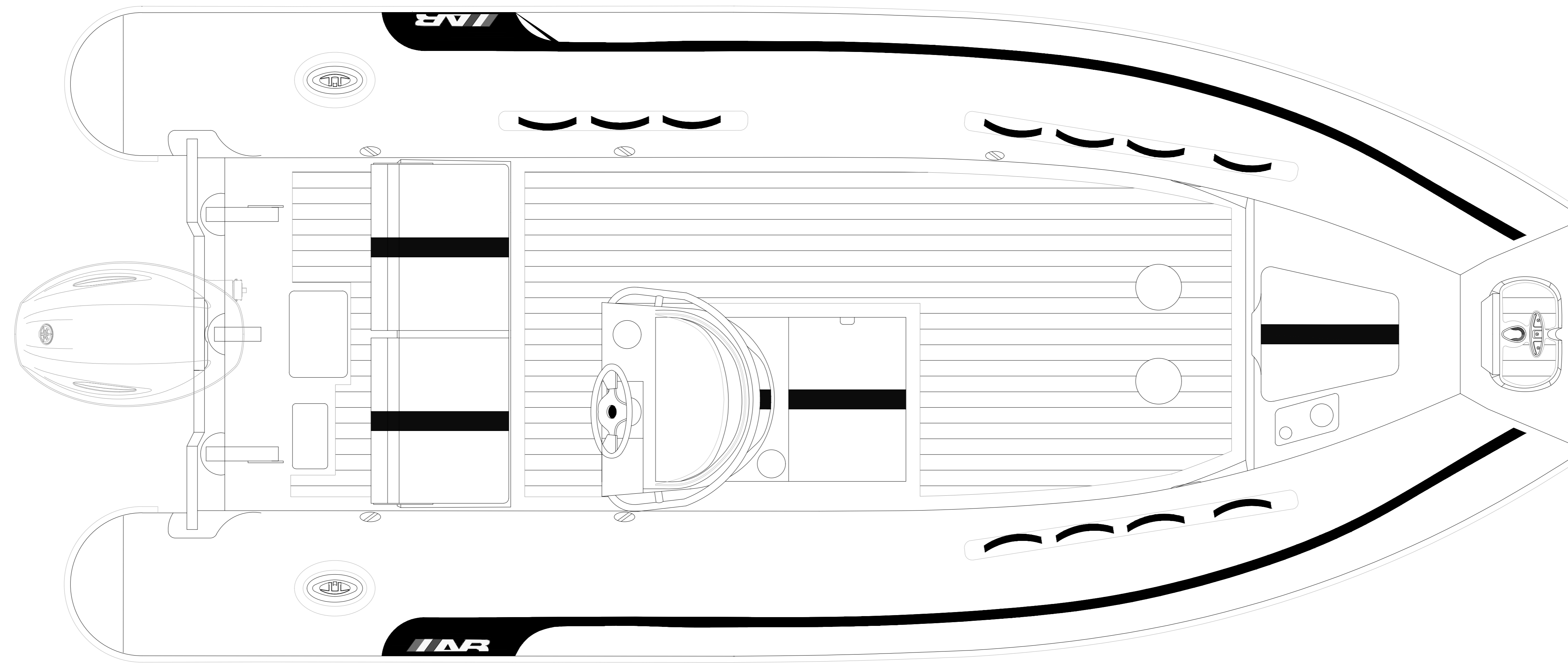
PLANT VIEW
