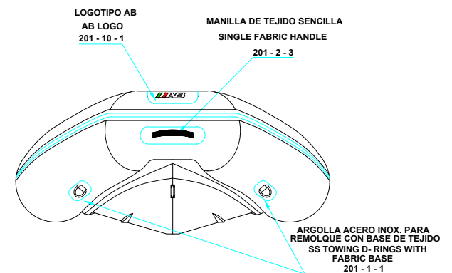
FORE VIEW VISTA FRONTAL
