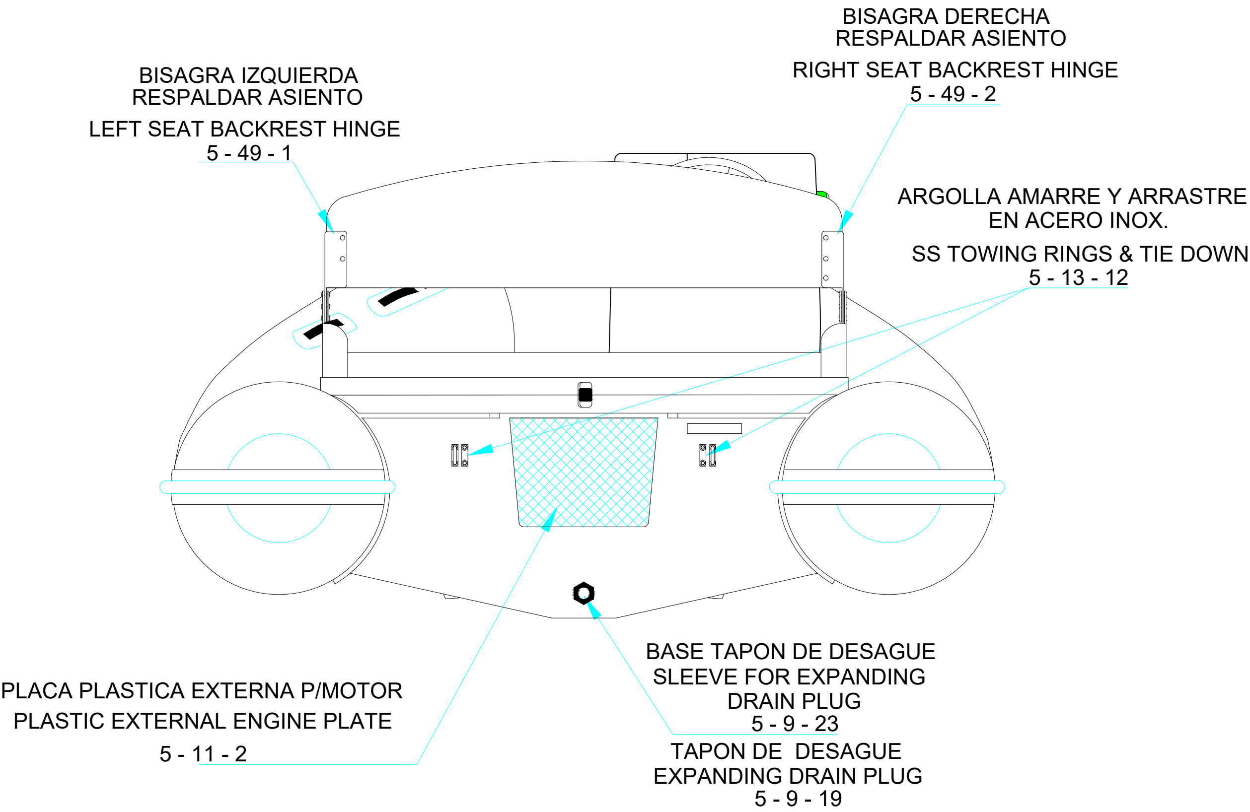
AFT VIEW VISTA TRASERA
