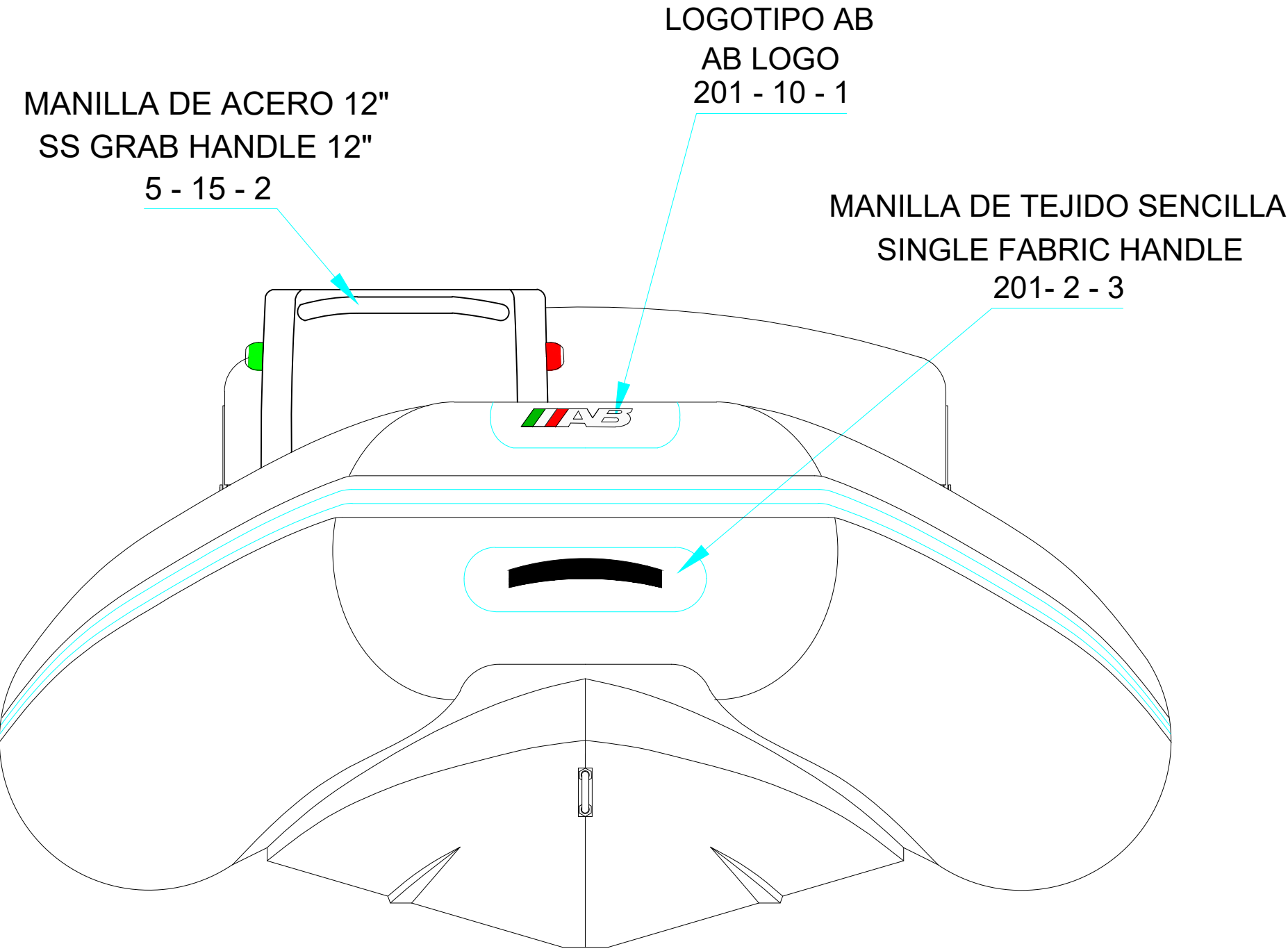
FORE VIEW VISTA FRONTAL
