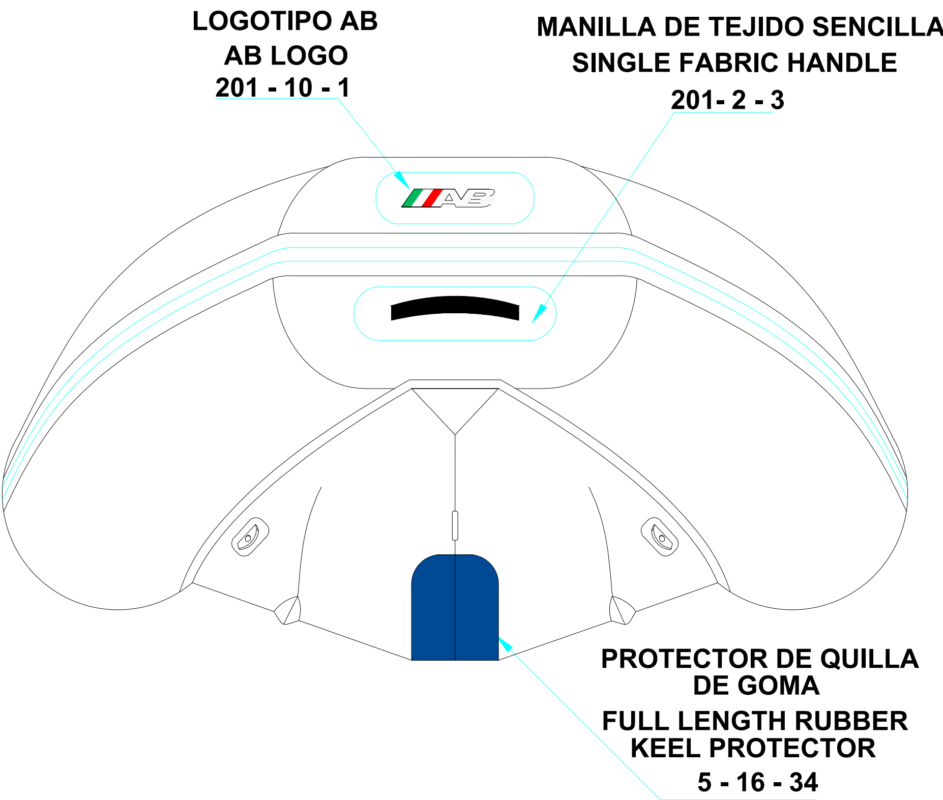
FORE VIEW VISTA FRONTAL
