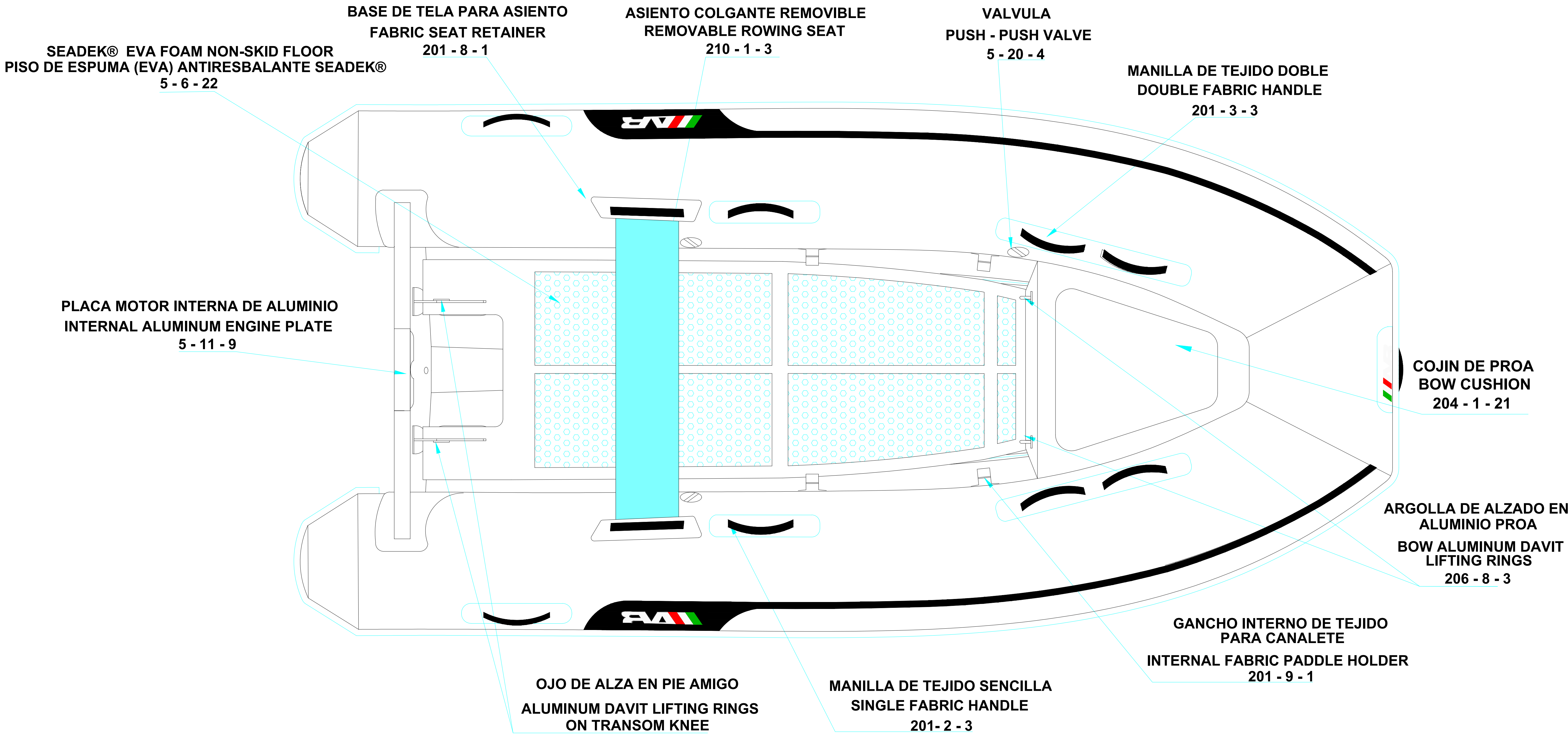
PLANT VIEW VISTA SUPERIOR
