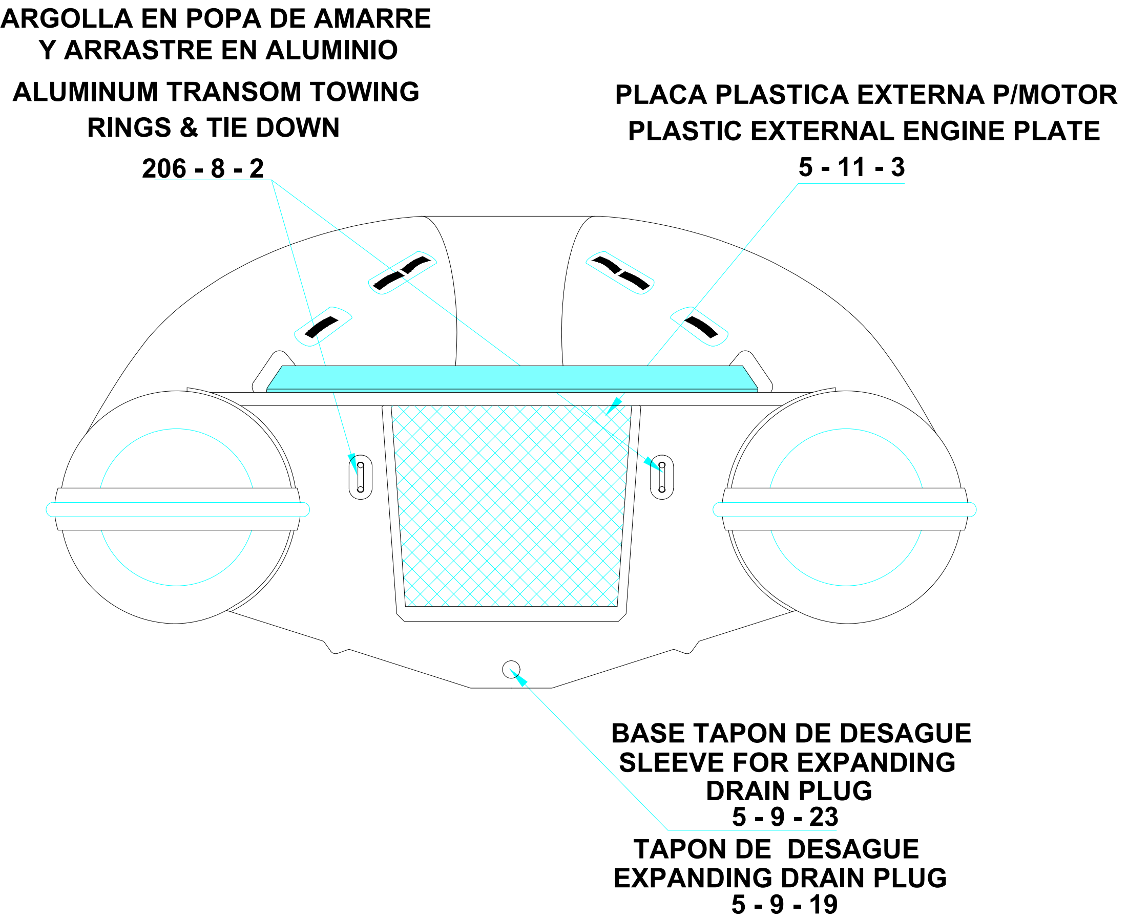
AFT VIEW VISTA TRASERA
