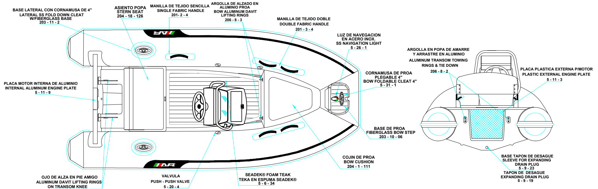
AFT VIEW VISTA TRASERA
