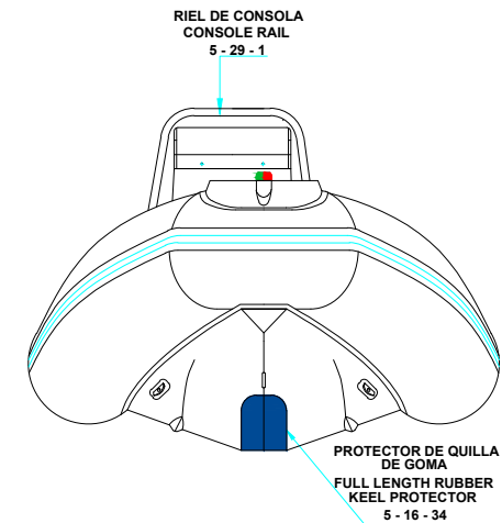
FORE VIEW VISTA FRONTAL
