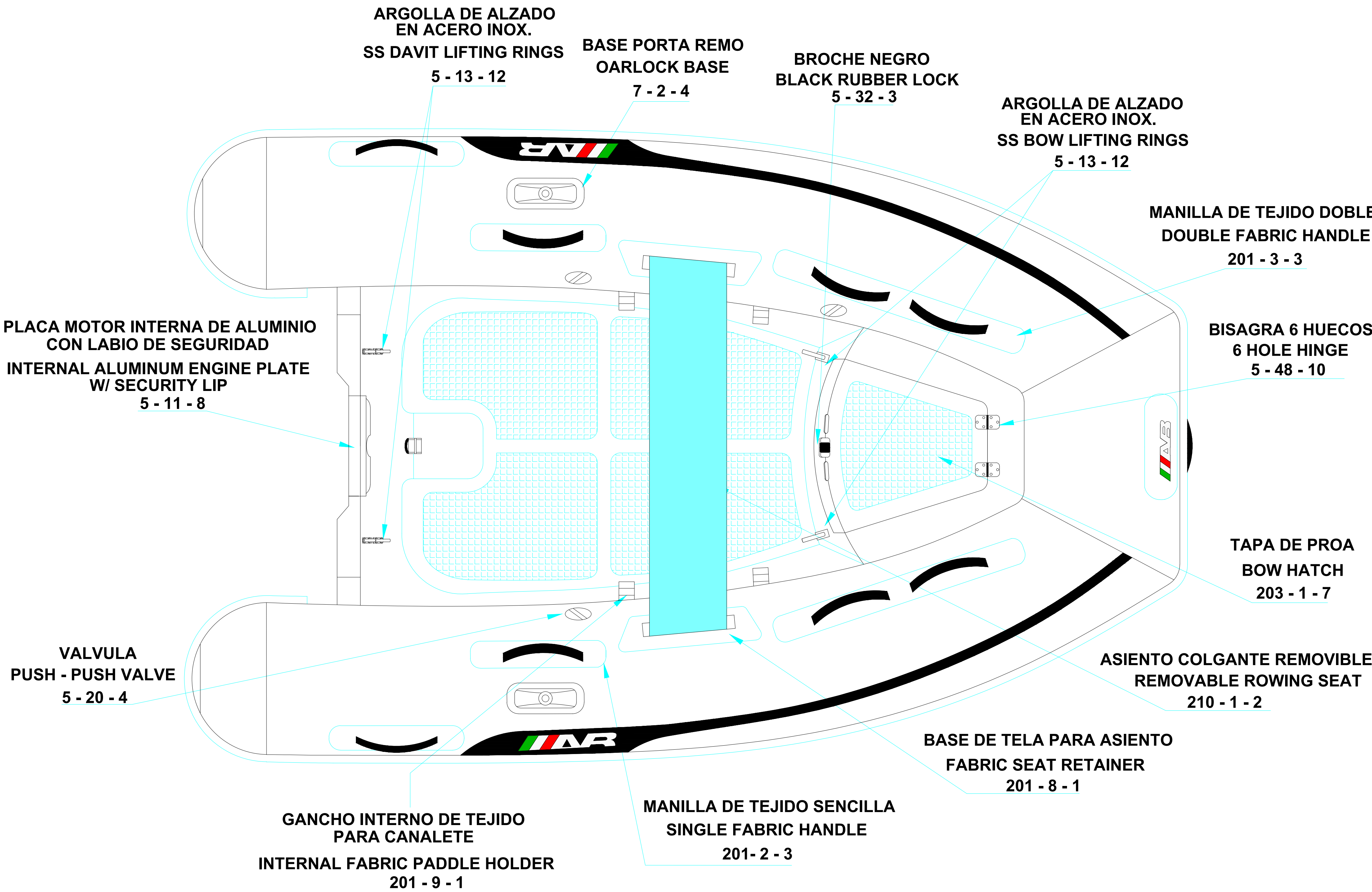
PLANT VIEW VISTA SUPERIOR
