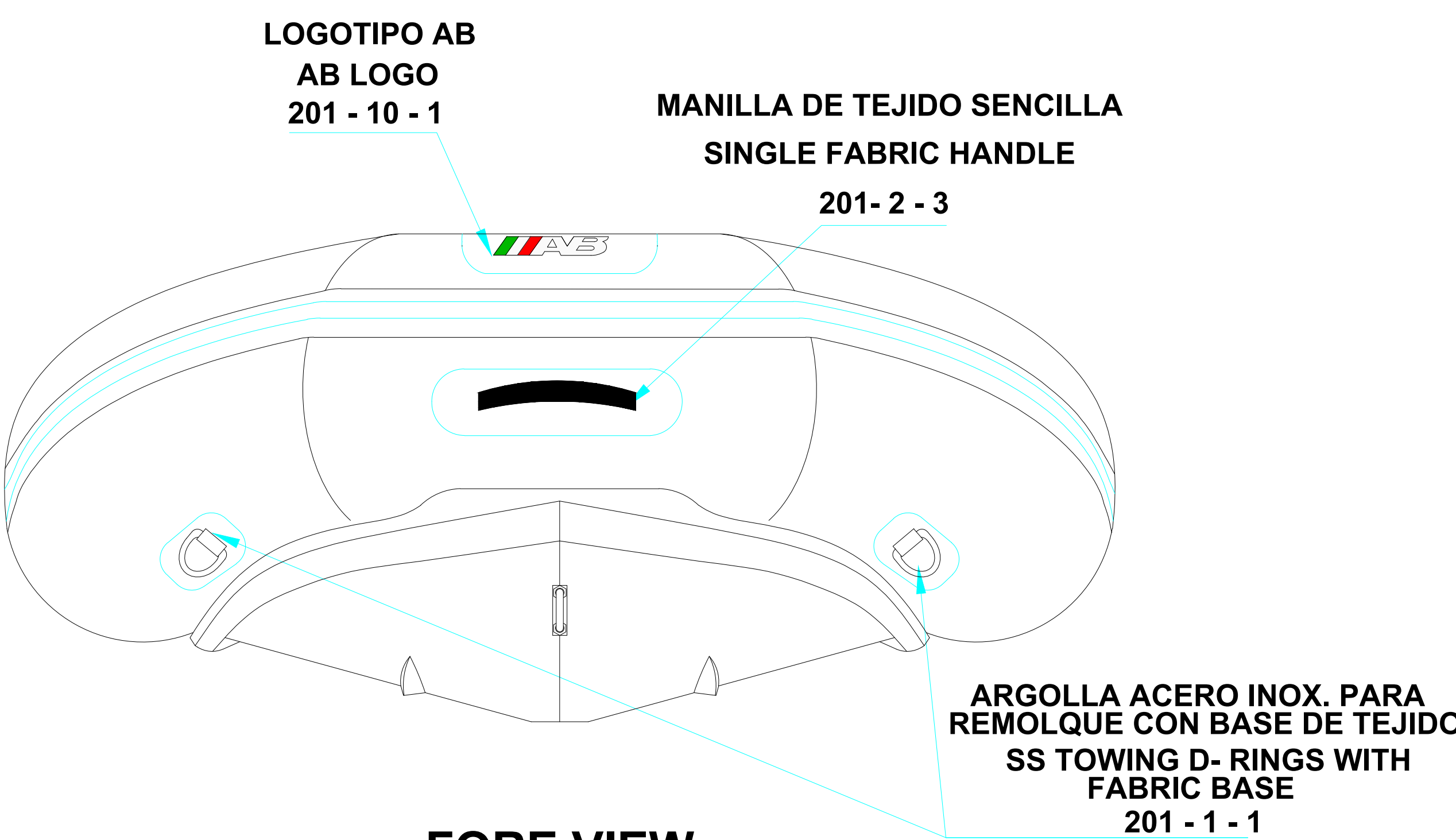
FORE VIEW VISTA FRONTAL
