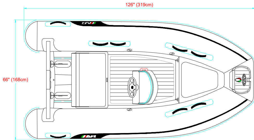
PLANT VIEW VISTA SUPERIOR
