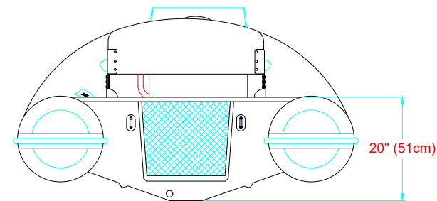
AFT VIEW VISTA TRASERA
