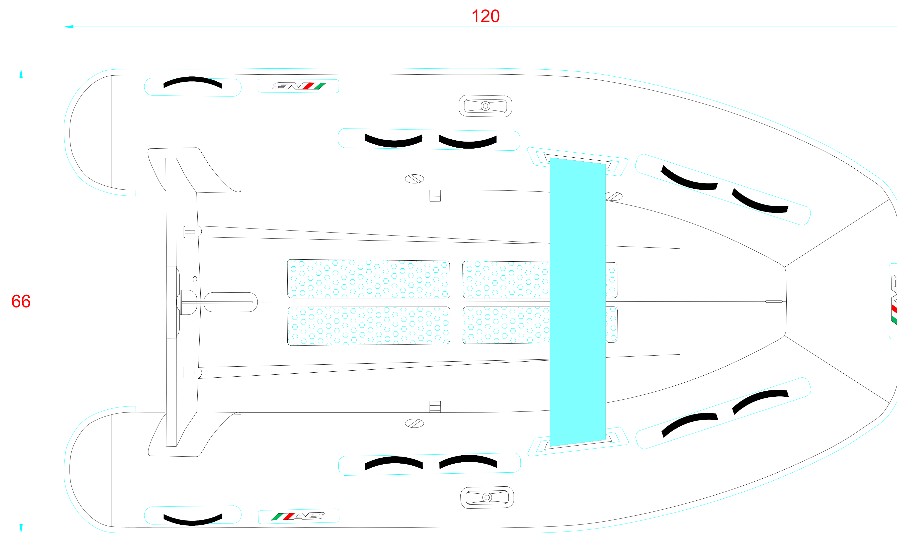
PLANT VIEW VISTA SUPERIOR
