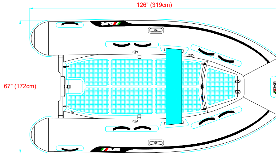
PLANT VIEW VISTA SUPERIOR
