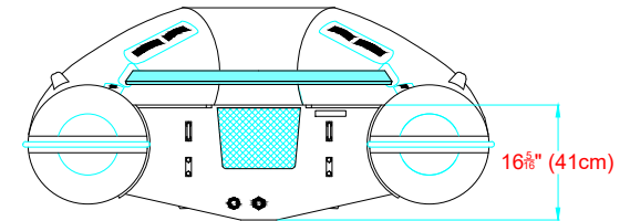
AFT VIEW VISTA TRASERA
