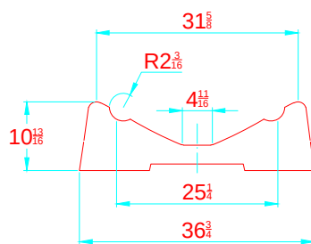
TRANSVERSAL SECTION "A" SECCION TRANSVERSAL "A"
