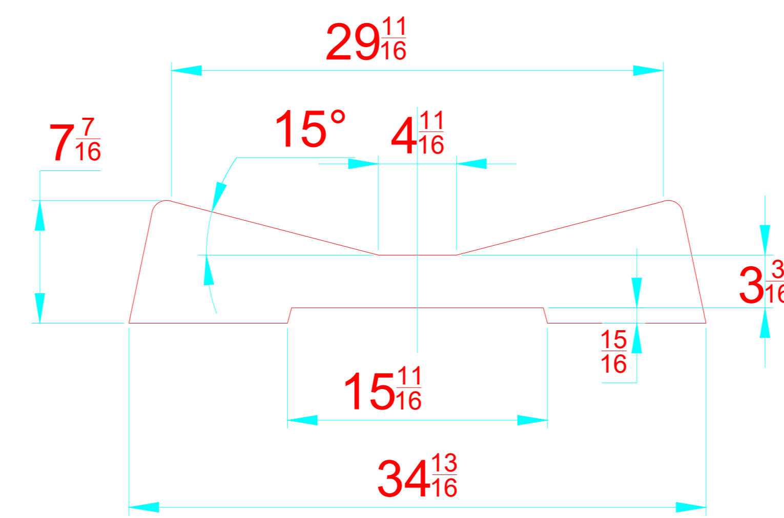
TRANSVERSAL SECTION "A" SECCION TRANSVERSAL "A"
