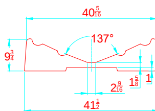
TRANSVERSAL SECTION "A" SECCION TRANSVERSAL "A"
