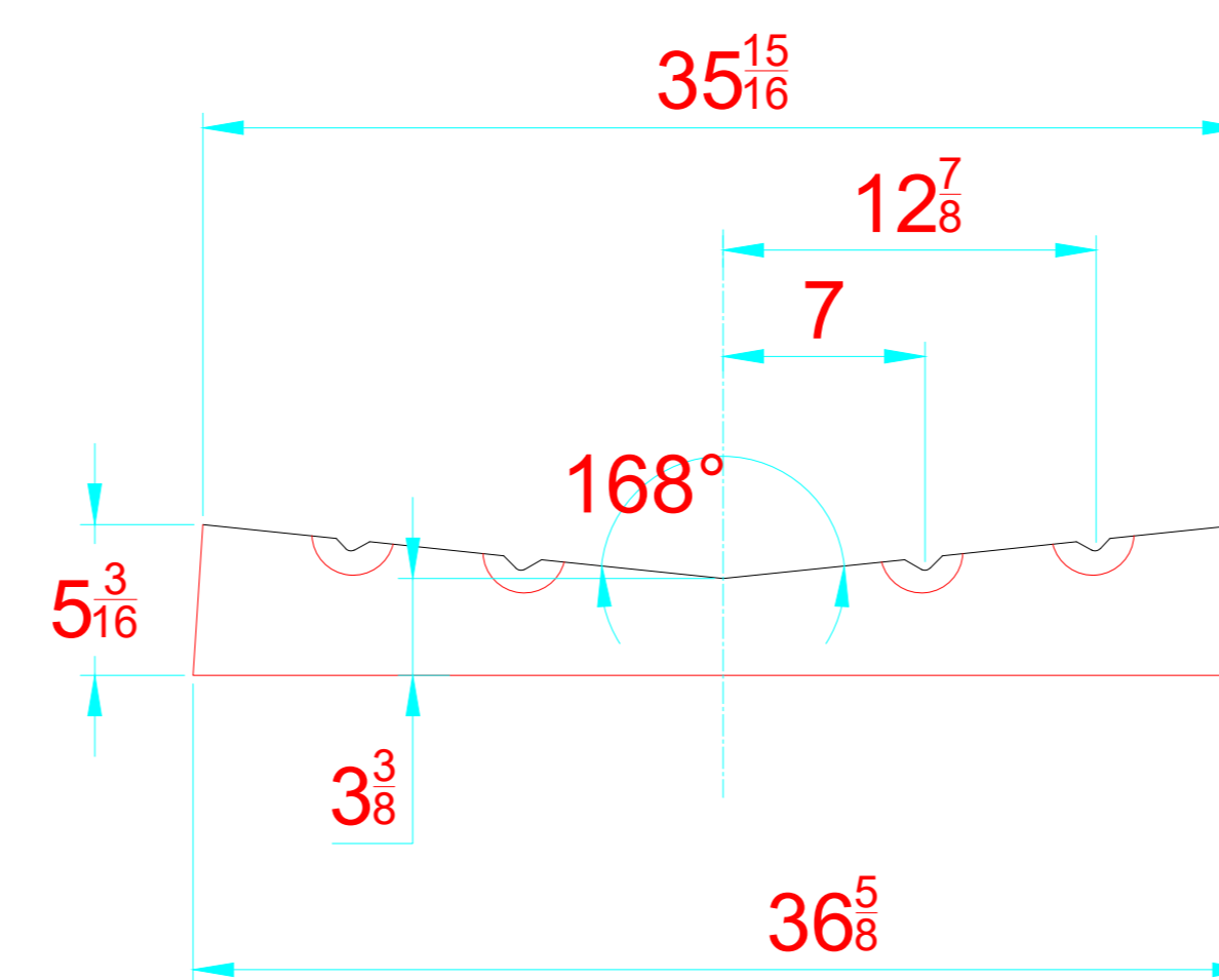
TRANSVERSAL SECTION "A" SECCION TRANSVERSAL "A"
