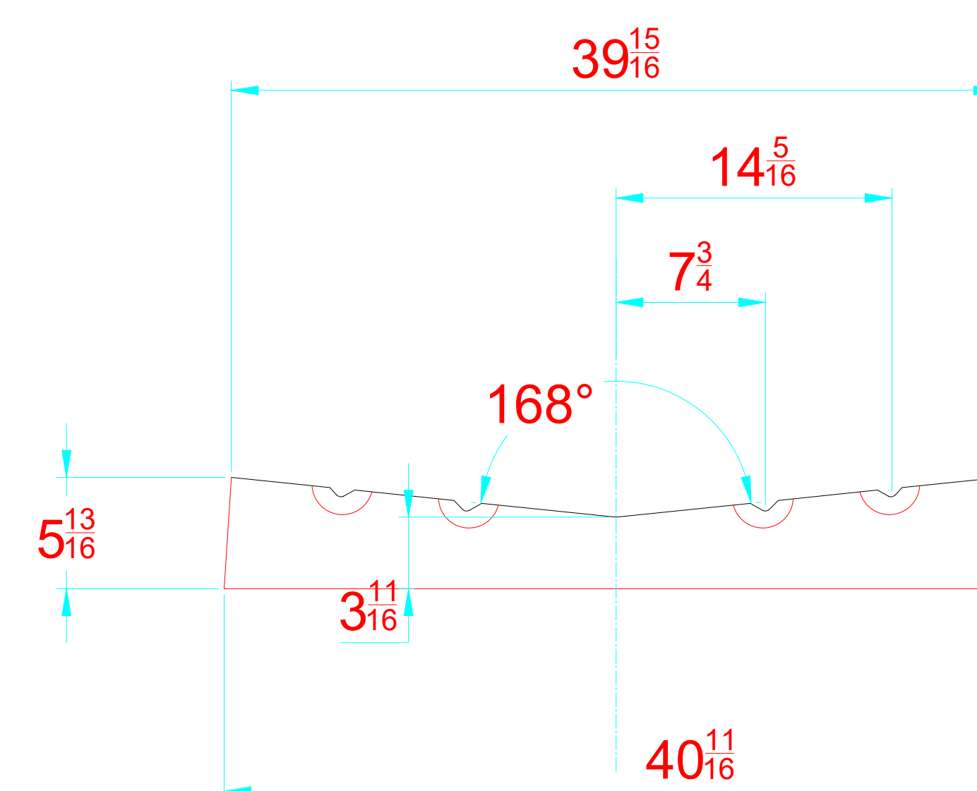
TRANSVERSAL SECTION "A" SECCION TRANSVERSAL "A"
