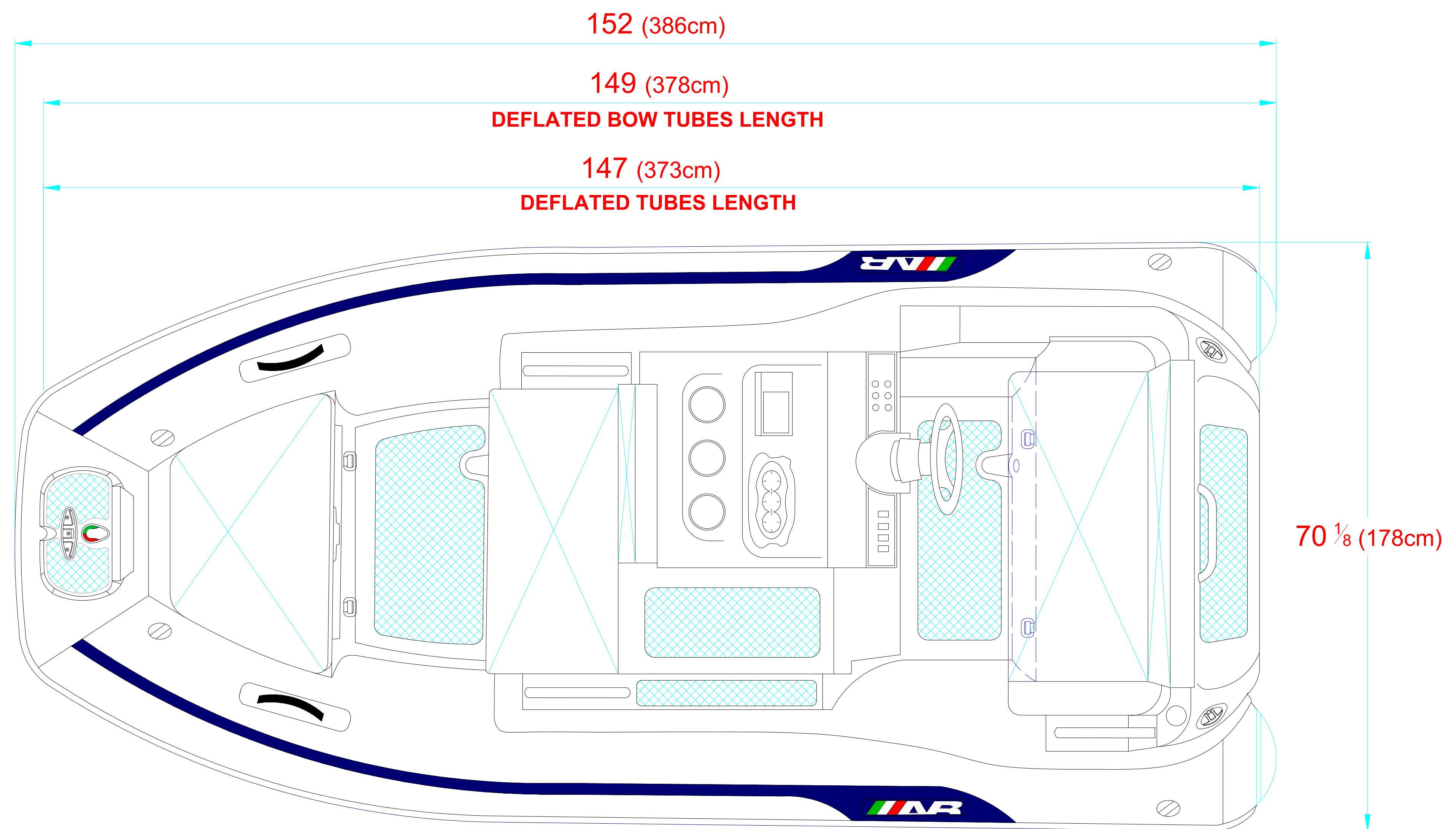
PLANT VIEW VISTA SUPERIOR
