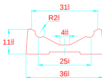
TRANSVERSAL SECTION "A" SECCION TRANSVERSAL "A"
