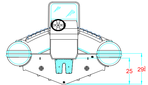
AFT VIEW VISTA TRASERA
