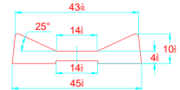
TRANSVERSAL SECTION "A" SECCION TRANSVERSAL "A"
