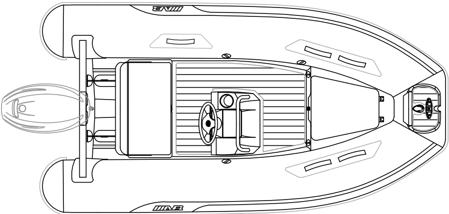
PLANT VIEW
