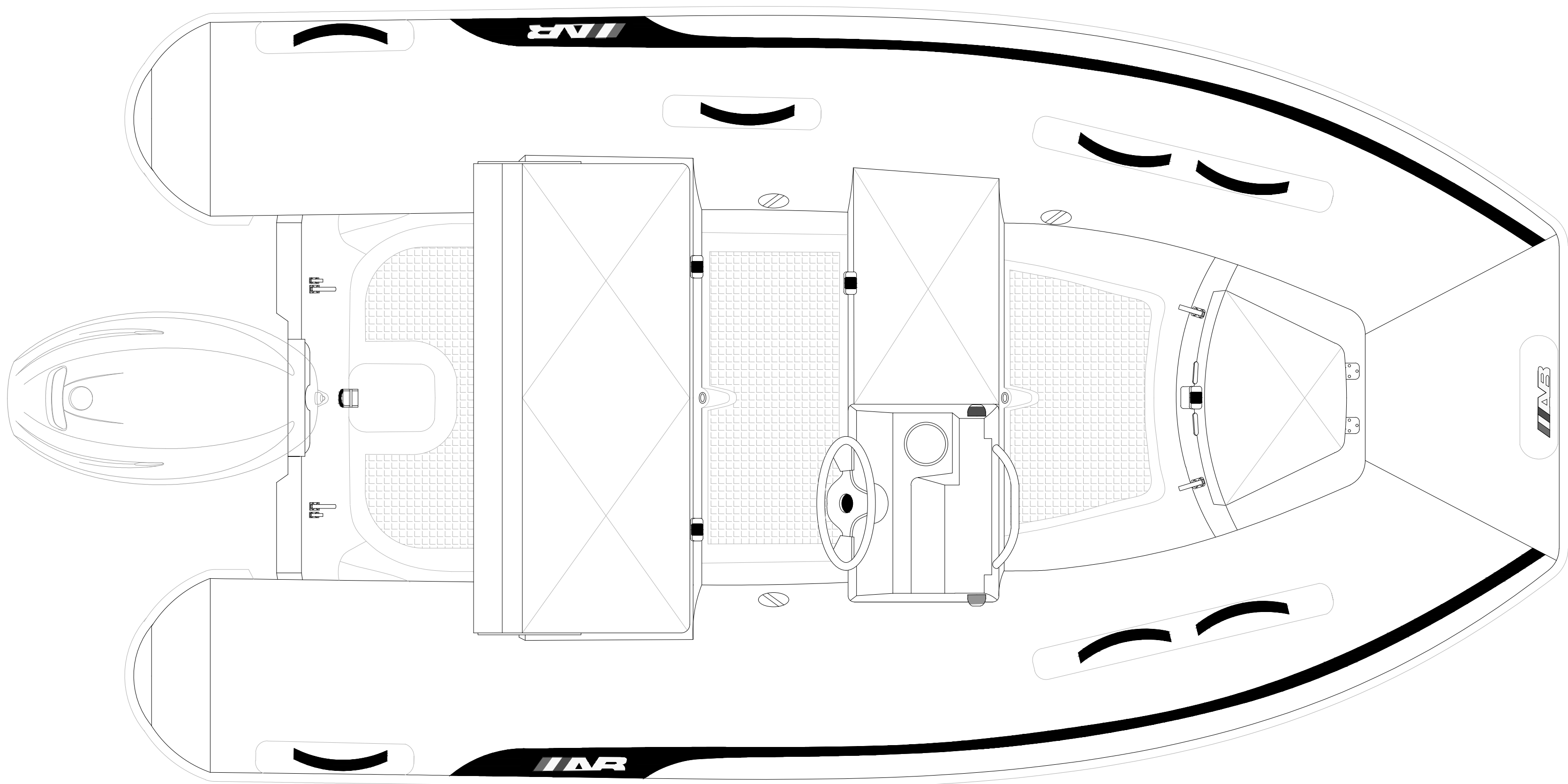
PLANT VIEW
