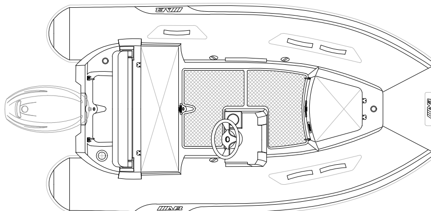
PLANT VIEW
