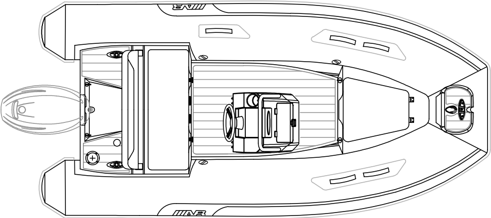
PLANT VIEW
