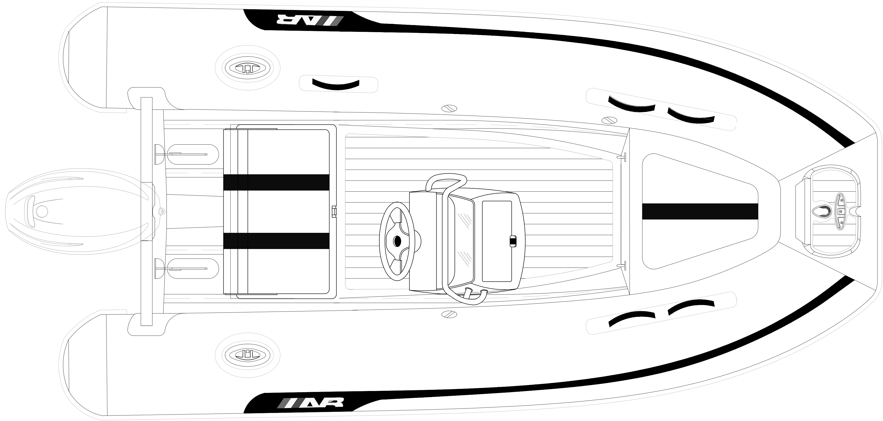
PLANT VIEW
