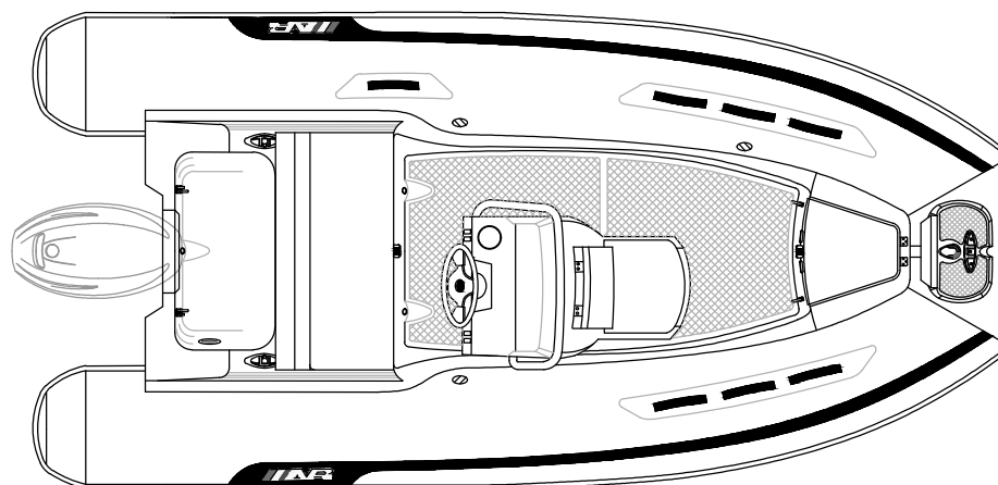
PLANT VIEW
