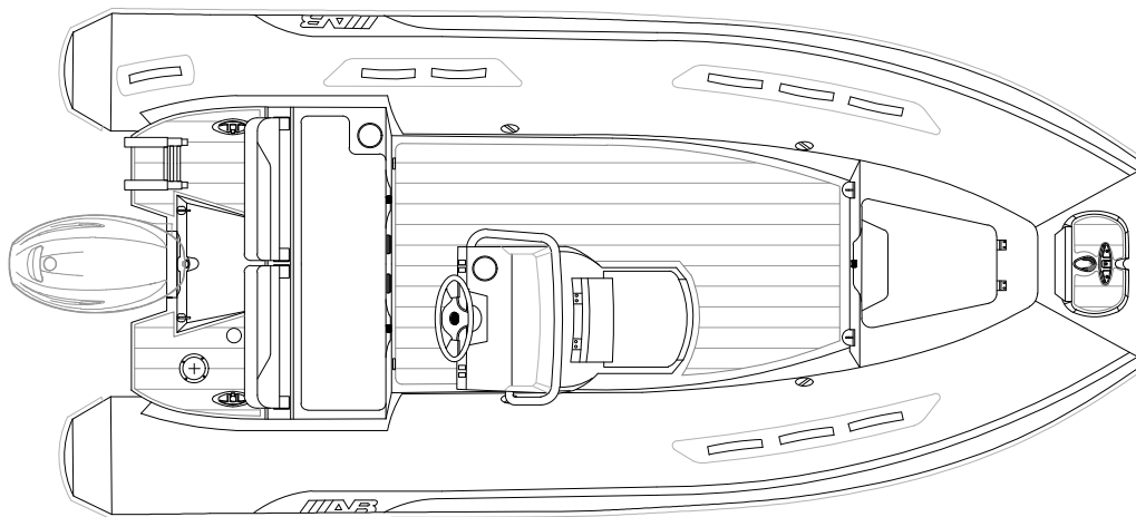
PLANT VIEW
