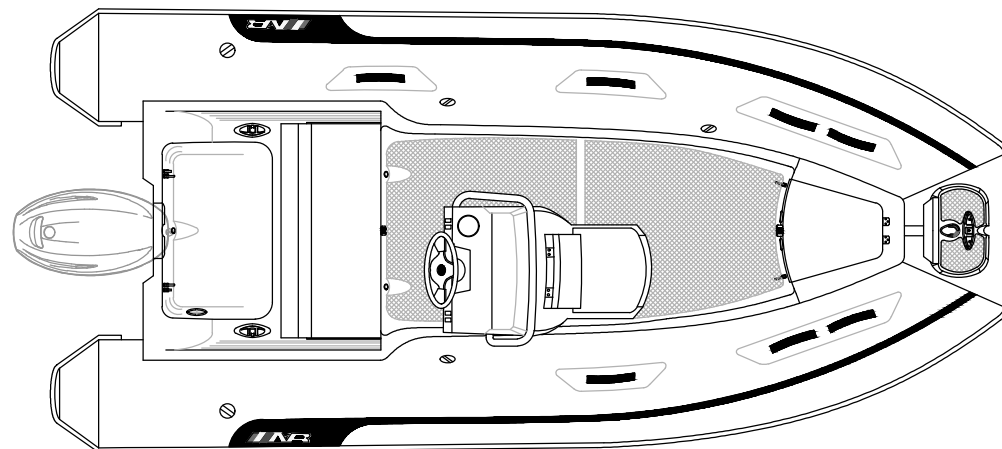
PLANT VIEW
