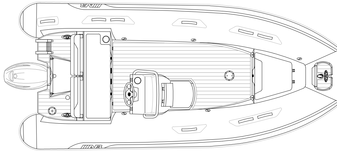
PLANT VIEW
