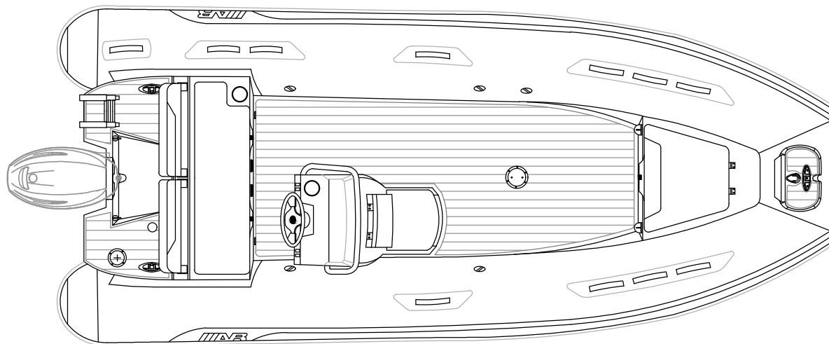
PLANT VIEW
