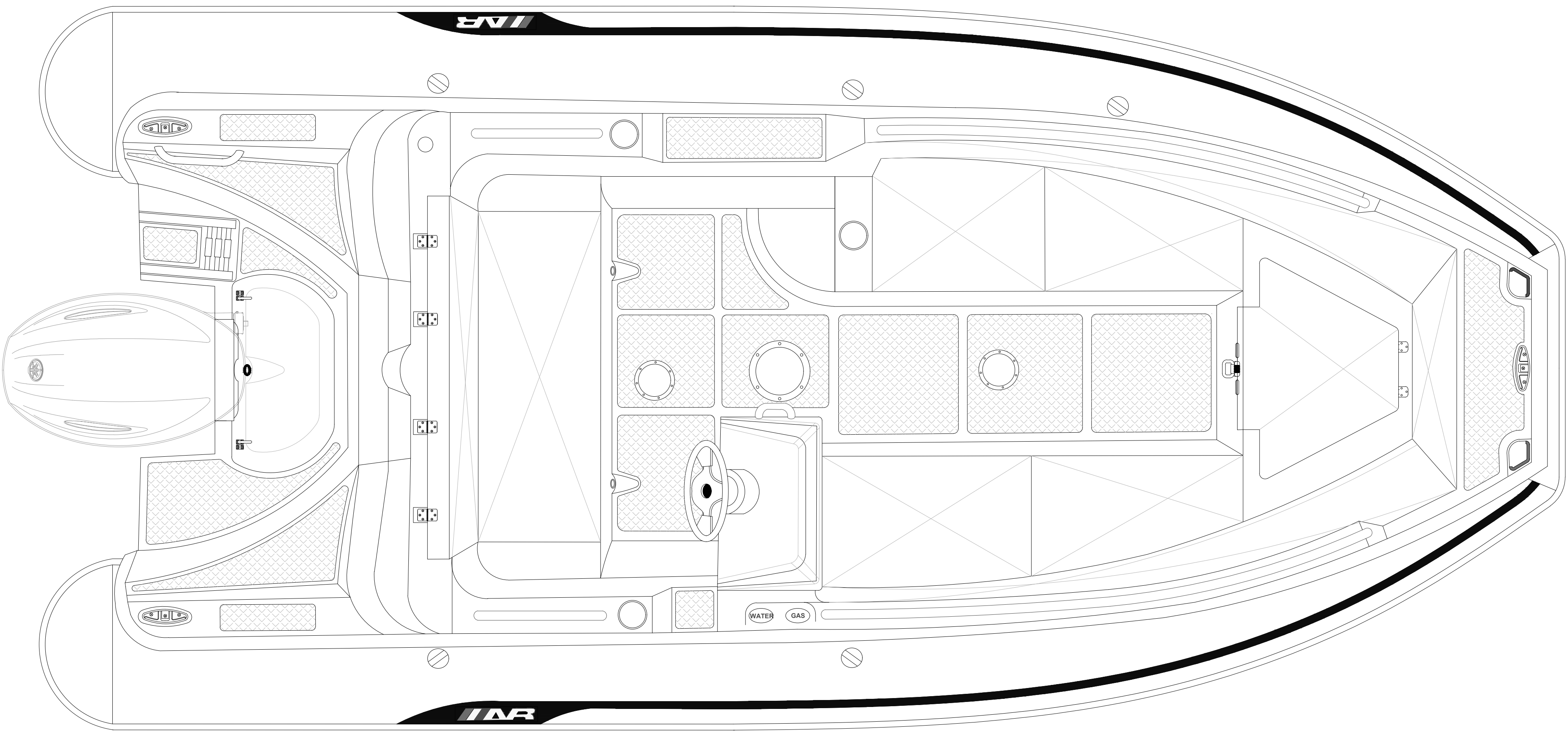
PLANT VIEW
