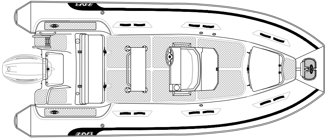
PLANT VIEW
