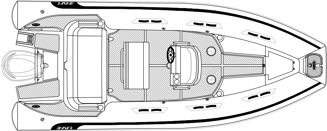
PLANT VIEW
