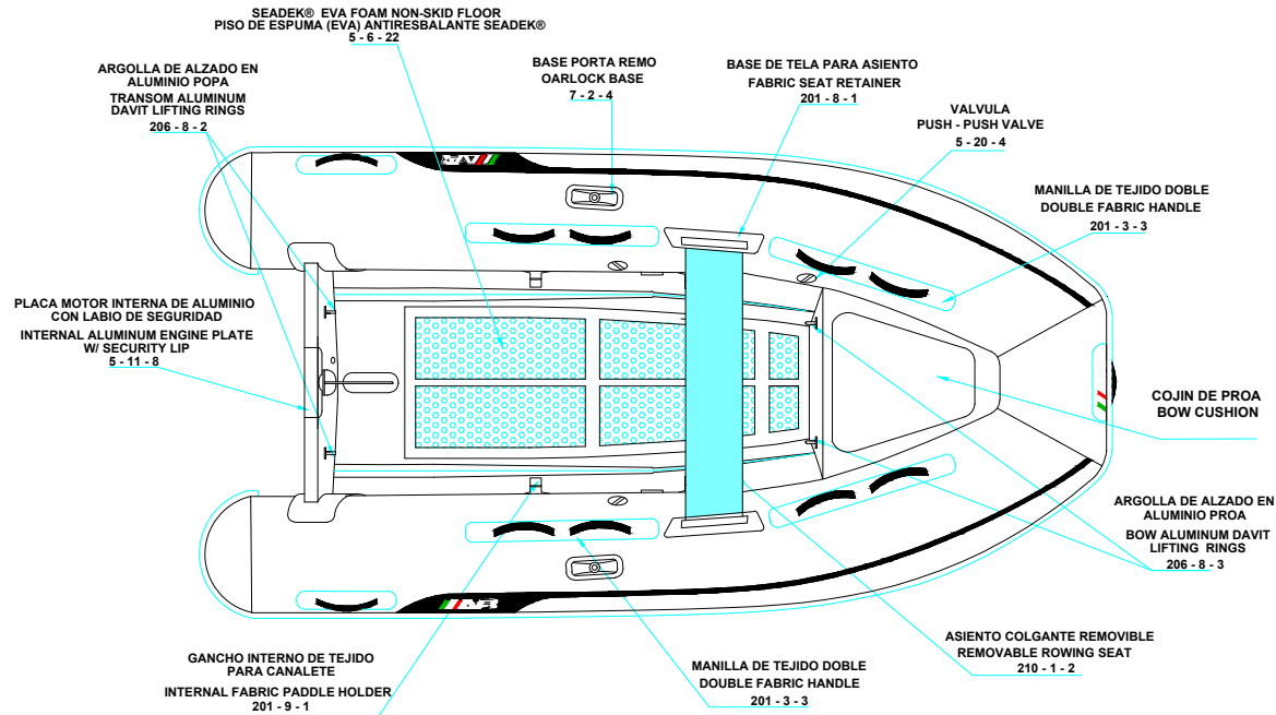
PLANT VIEW VISTA SUPERIOR
