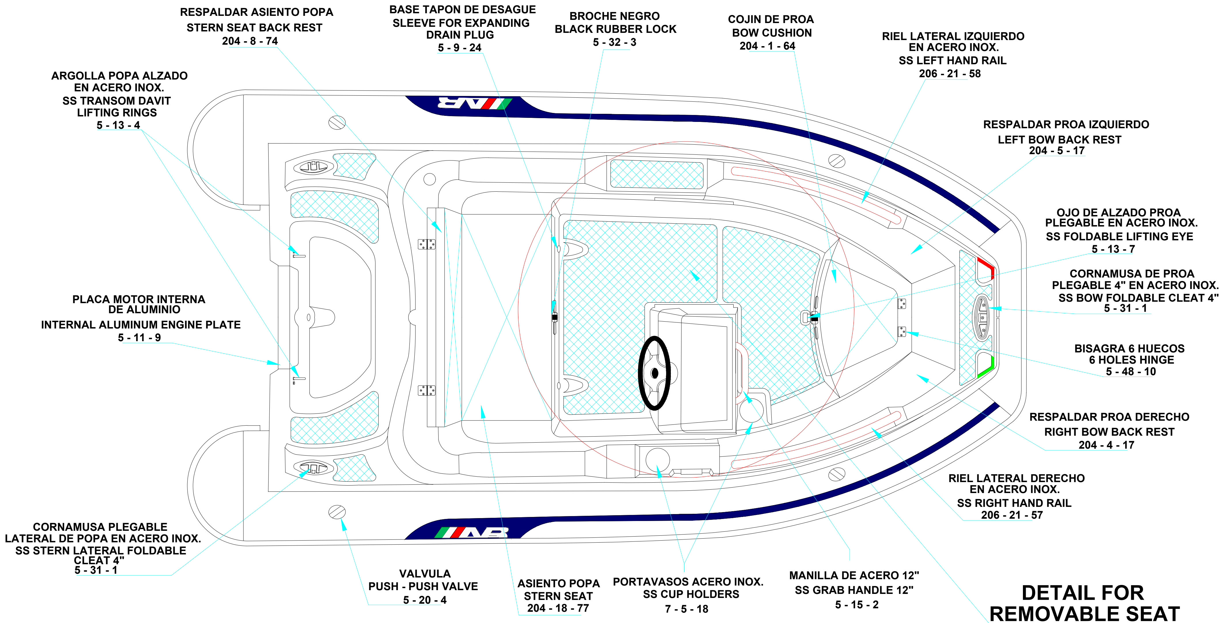
PLANT VIEW VISTA SUPERIOR
