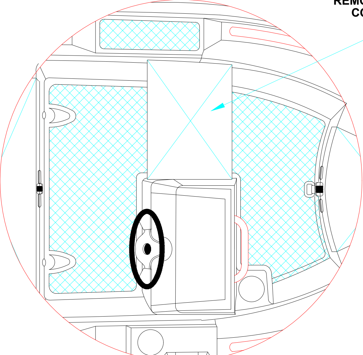
DETAIL FOR REMOVABLE SEAT
