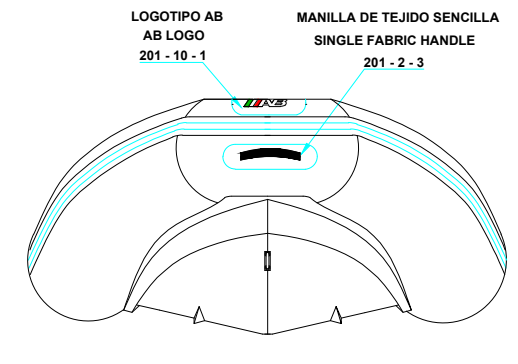
FORE VIEW VISTA FRONTAL
