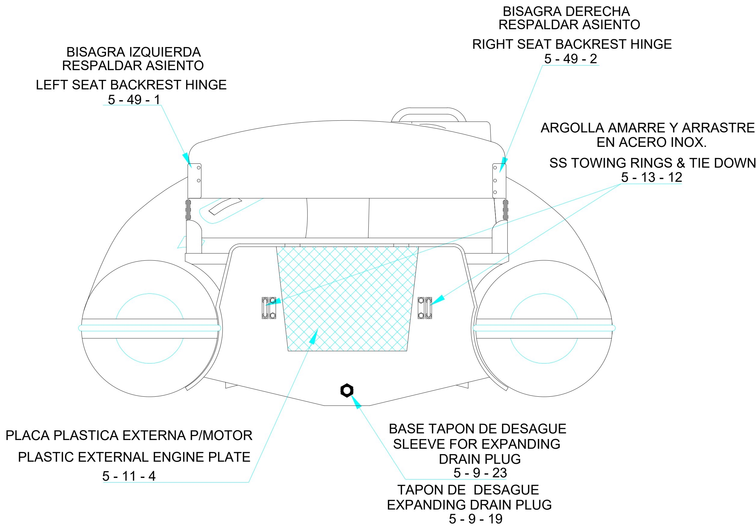
AFT VIEW VISTA TRASERA
