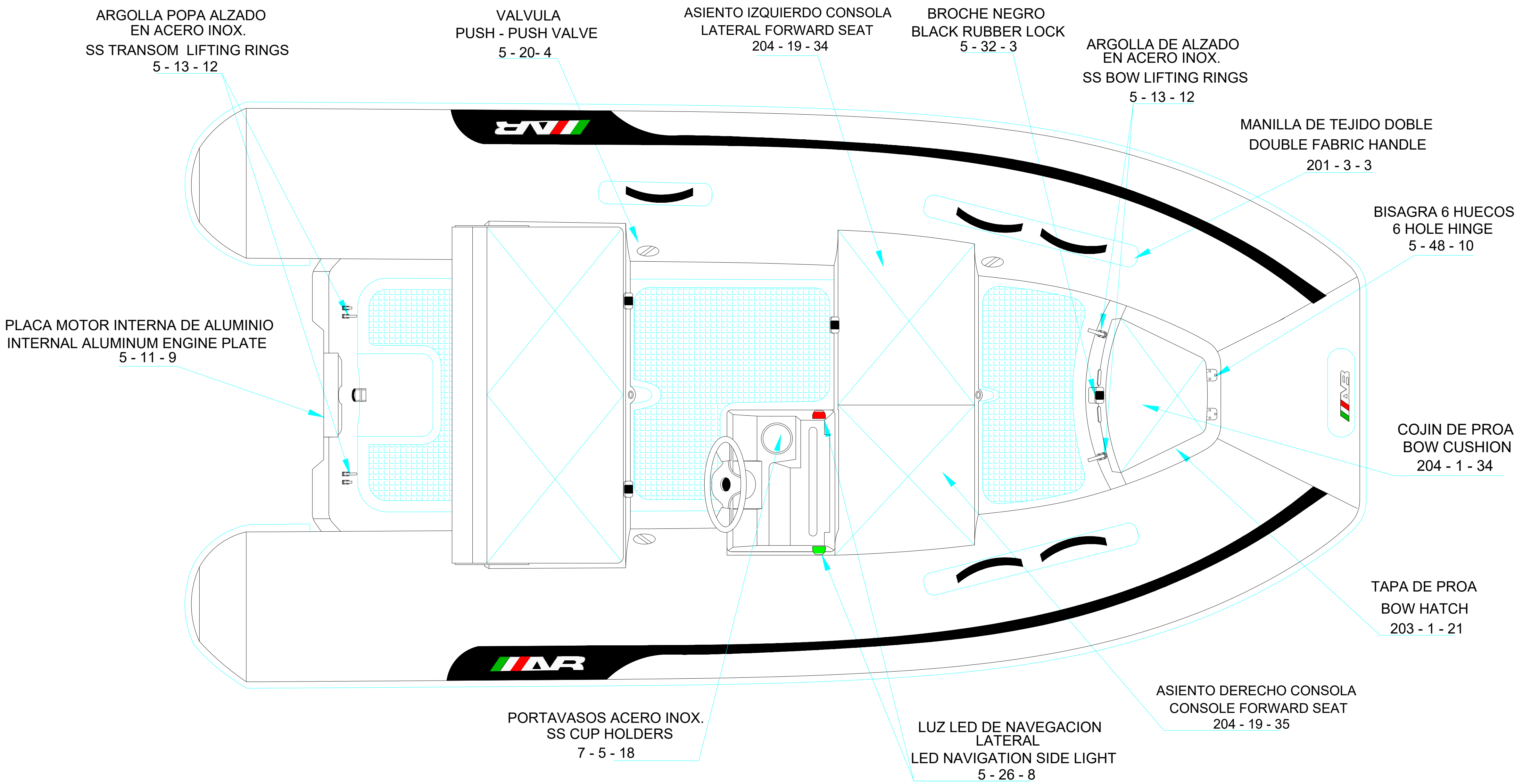
PLANT VIEW VISTA SUPERIOR
