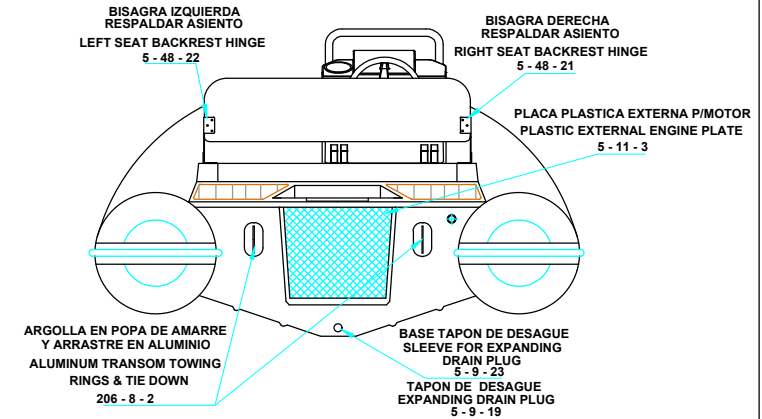
AFT VIEW VISTA TRASERA
