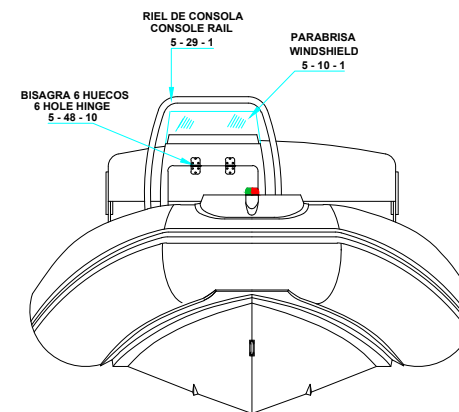
FORE VIEW VISTA FRONTAL
