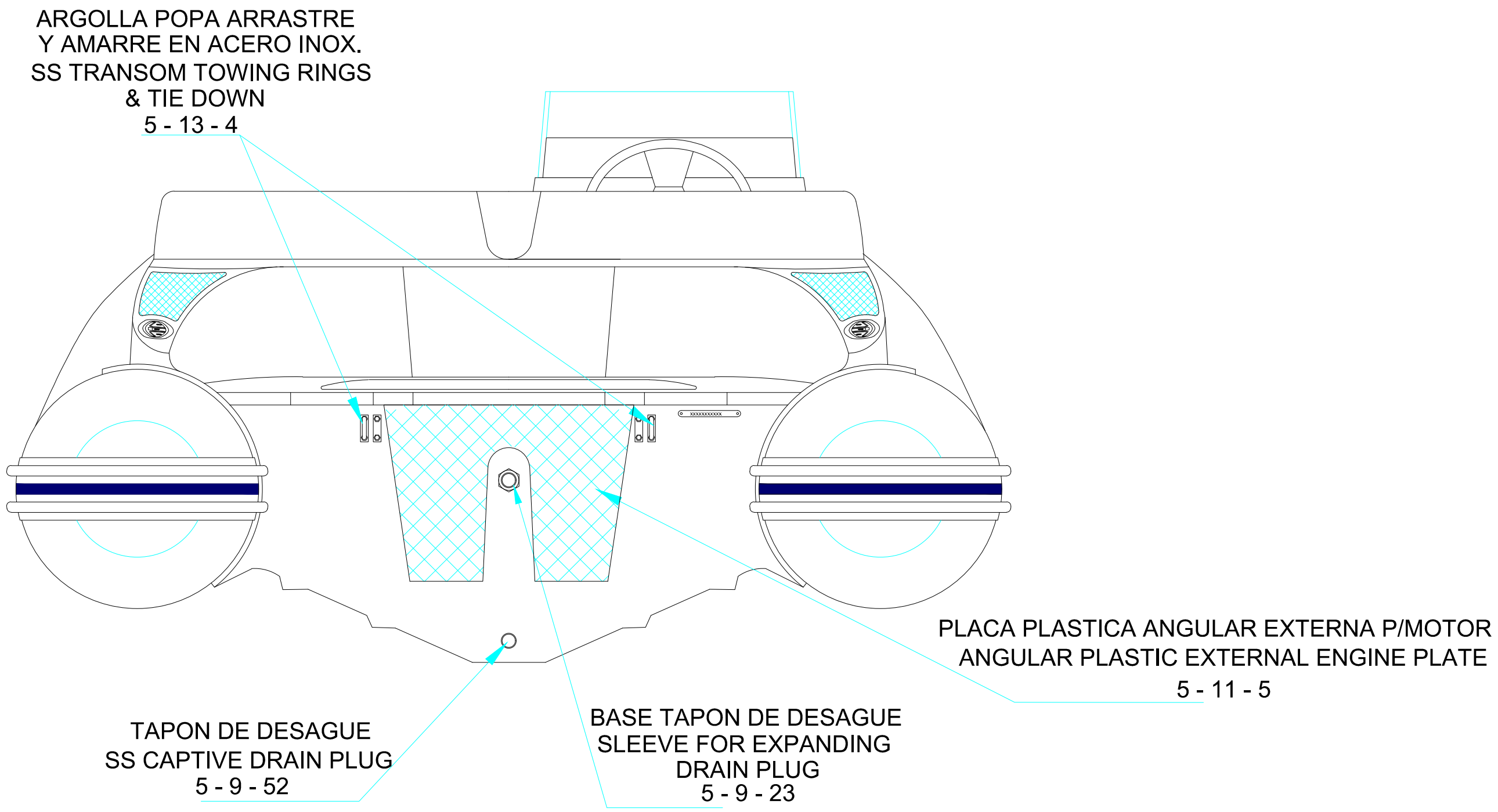
AFT VIEW VISTA TRASERA
