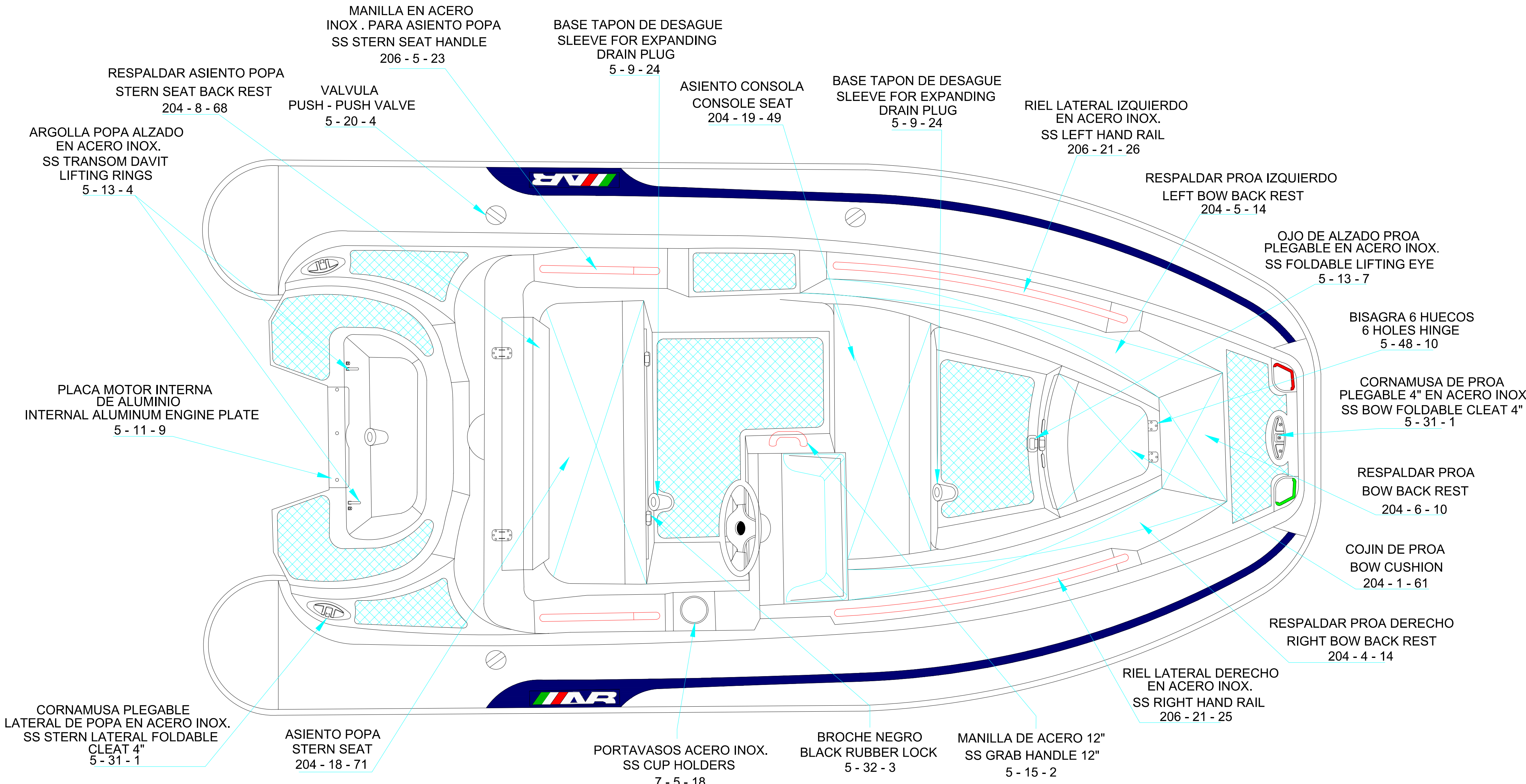
PLANT VIEW VISTA SUPERIOR
