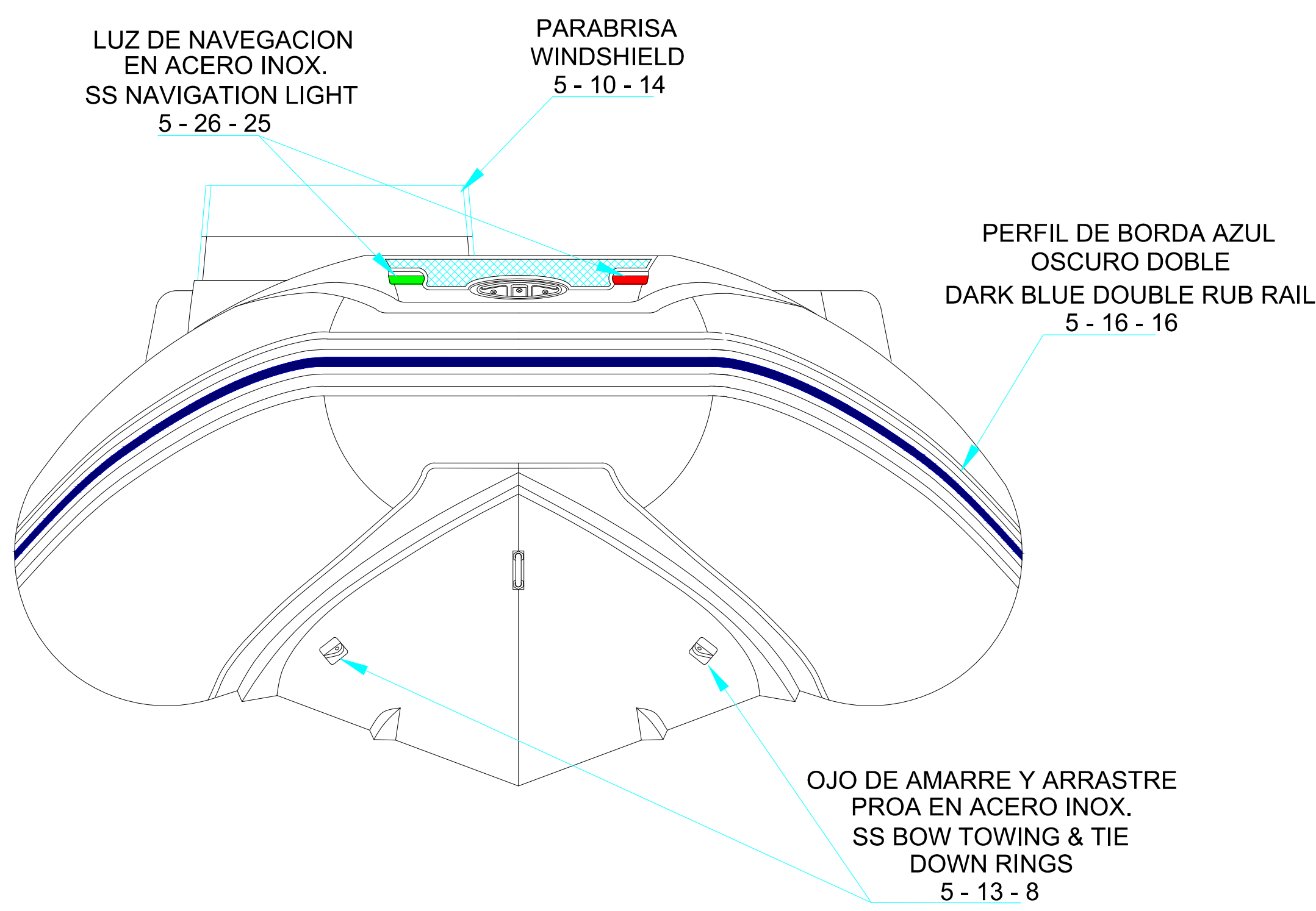
FORE VIEW VISTA FRONTAL
