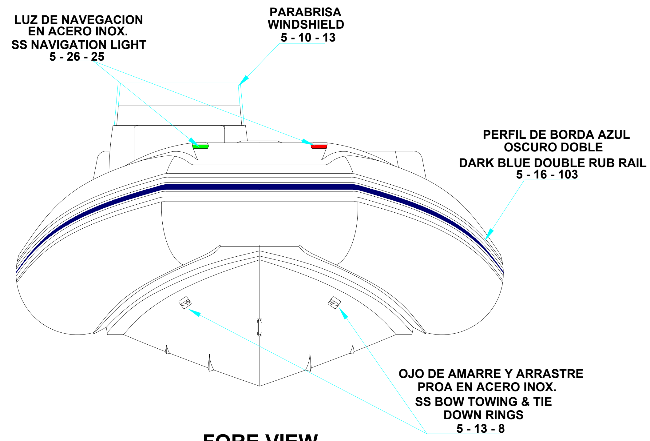
FORE VIEW VISTA FRONTAL
