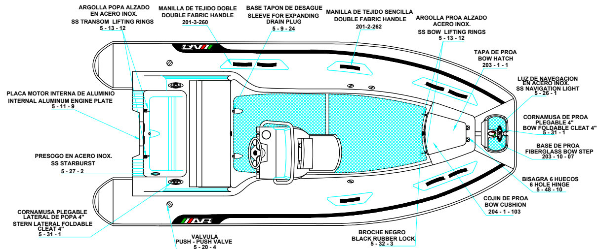
PLANT VIEW VISTA SUPERIOR
